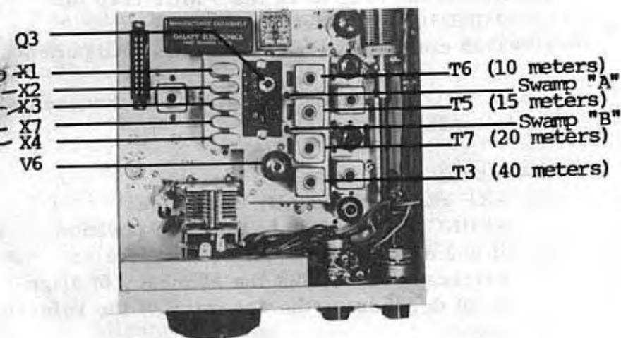
CONVERTER ALIGNMENT IDENTIFICATION
