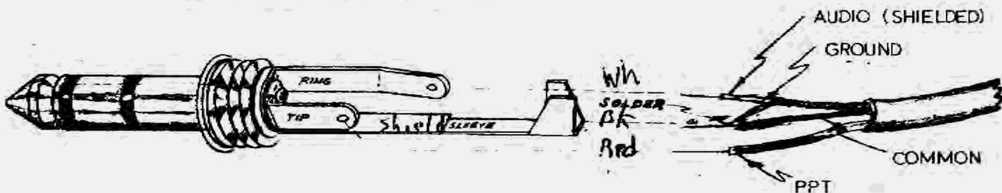
MICROPHONE CONNECTION
