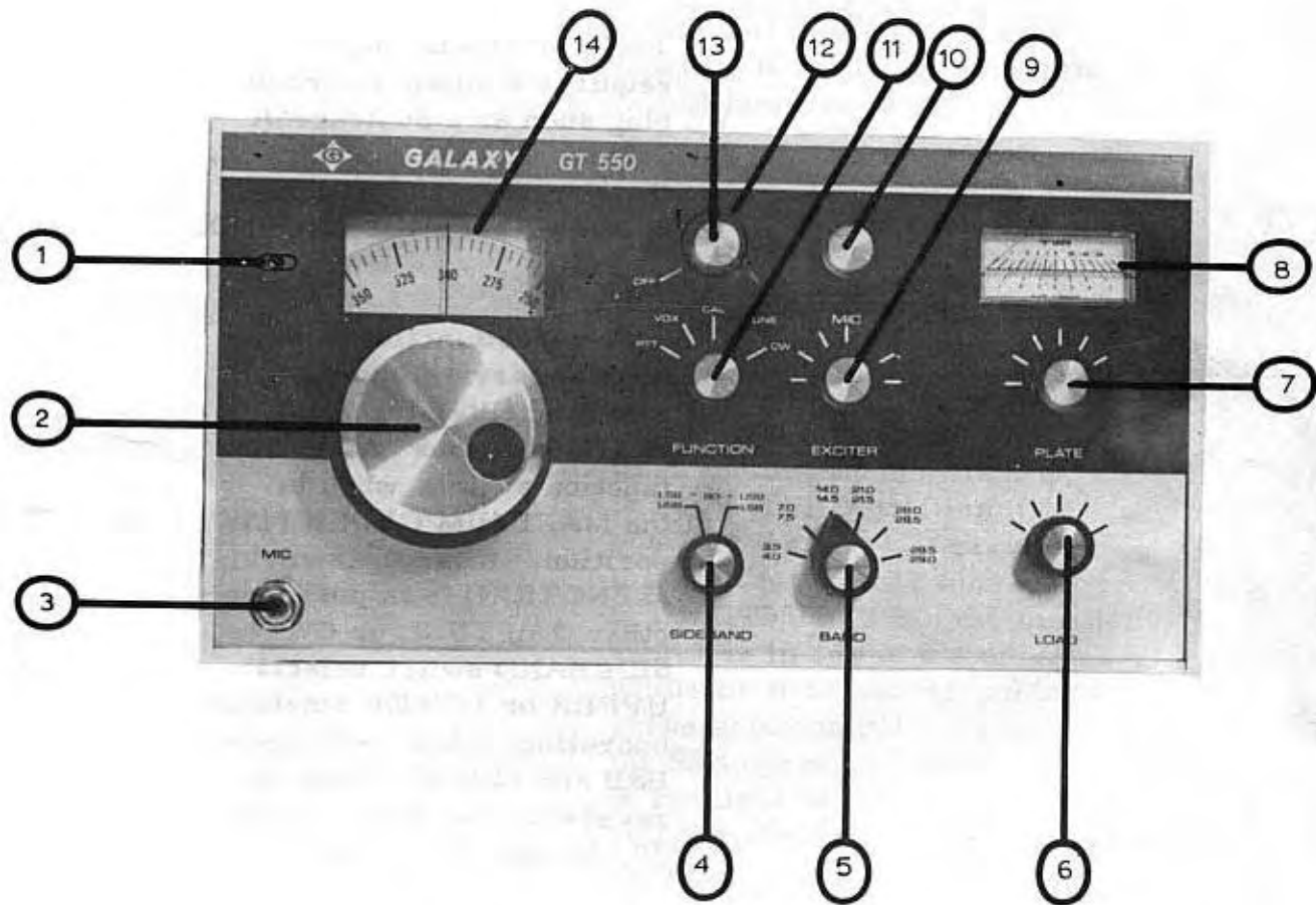
FRONT-VIEW OF THE GT550
